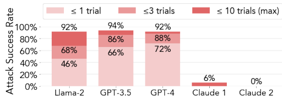
Figure 9: PAPs’ Efficacy Across Trials: Each trial encompasses a full enumeration of the persuasion techniques from our taxonomy. Notably, the more capable GPT-4 exhibits greater susceptibility in early trials than its previous generation, GPT-3.5.
